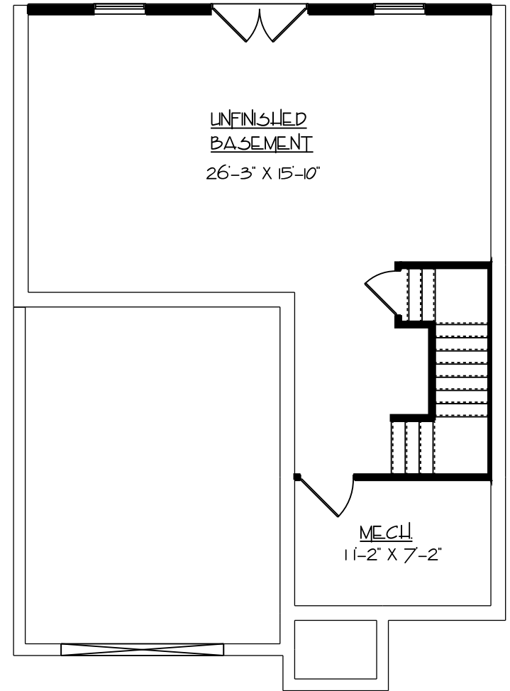
FOUNDATION PLAN
