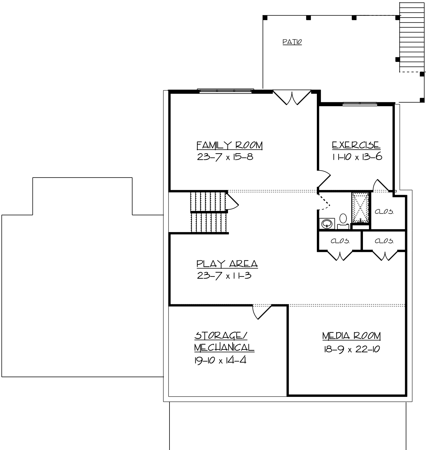
"BRADFORD" FOUNDATION PLAN
