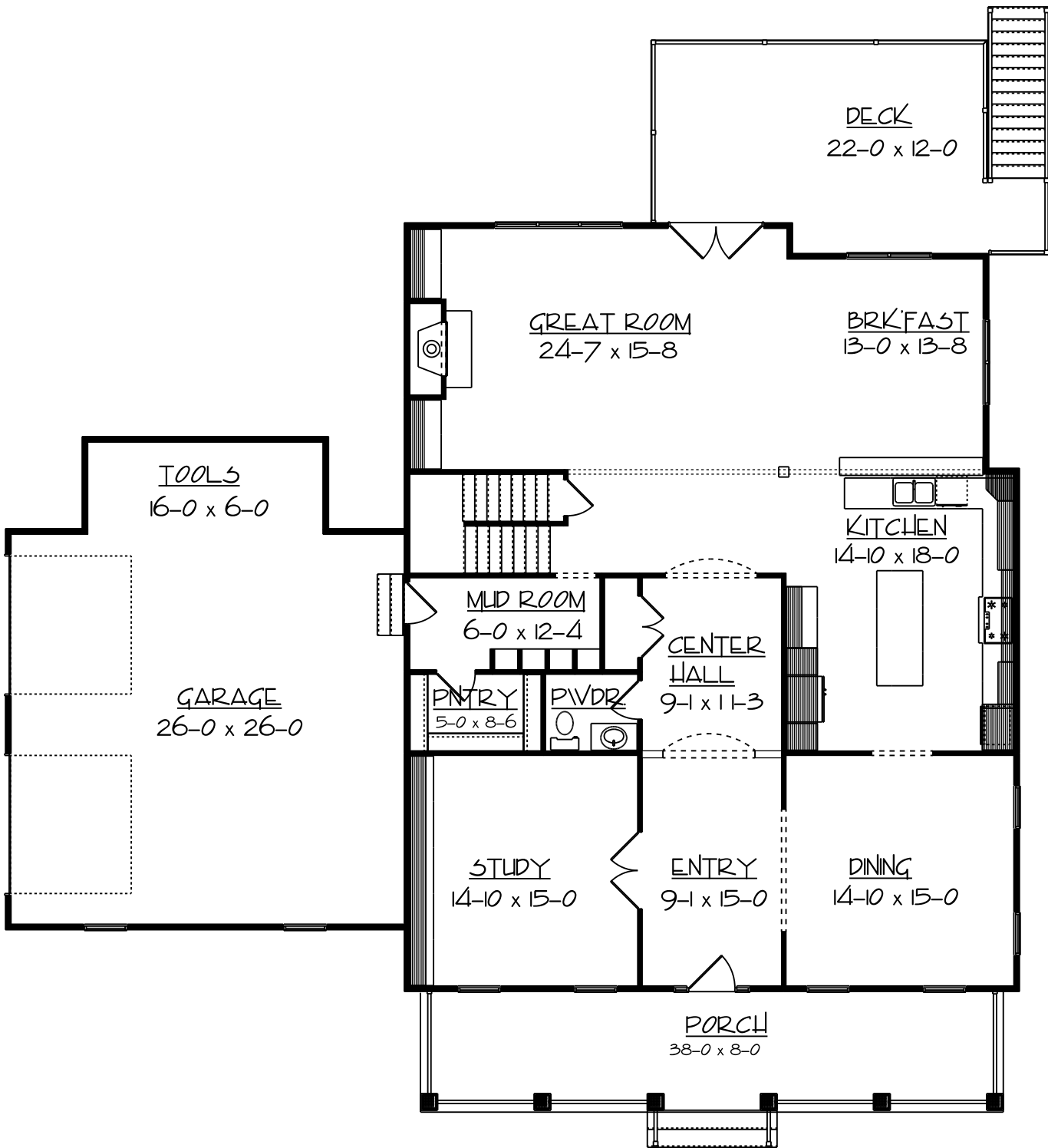
"BRADFORD" FIRST FLOOR PLAN
