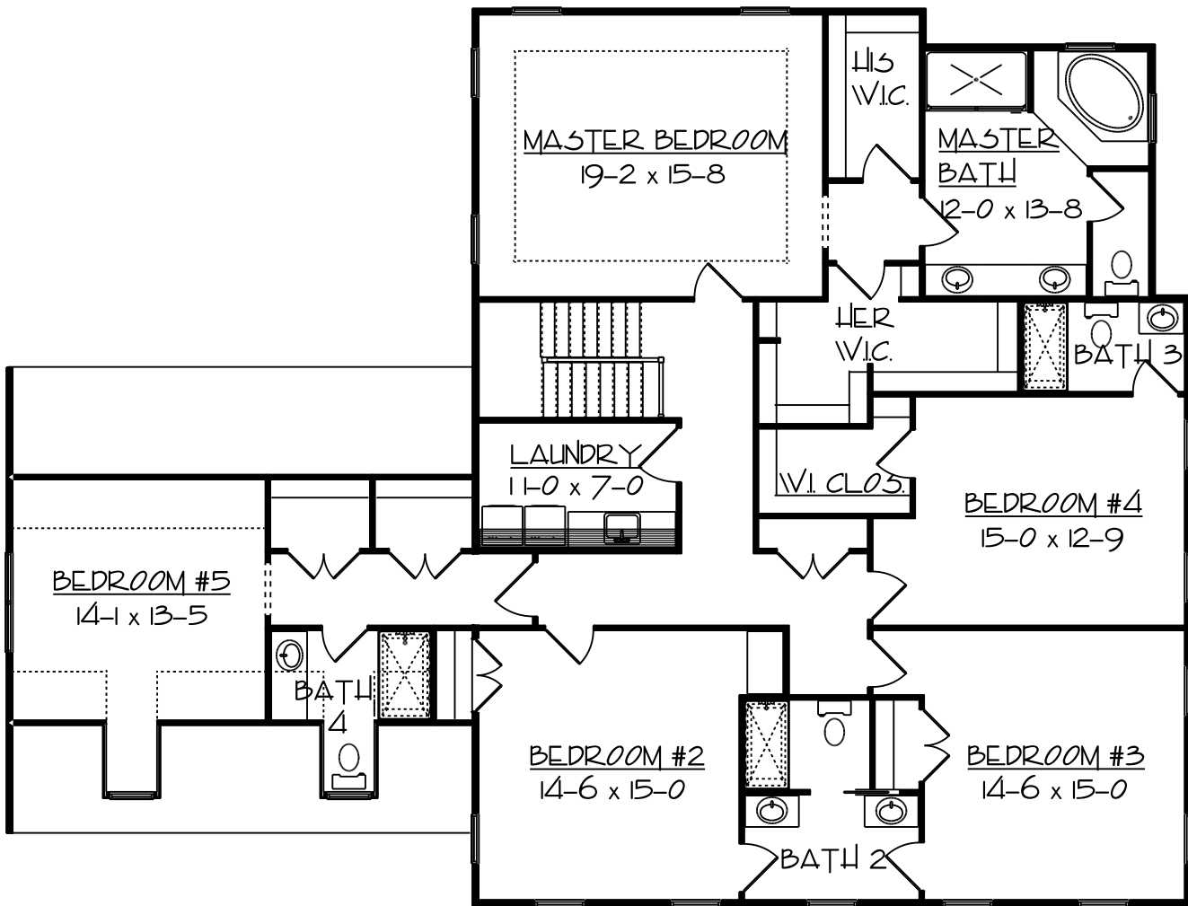
"BRADFORD" SECOND FLOOR PLAN
